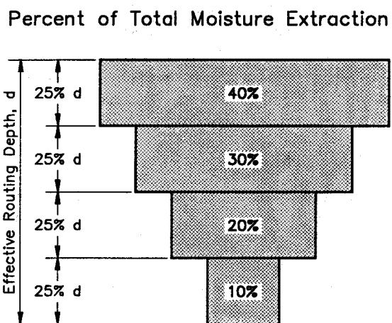
Figure 4. The basic soil moisture extraction pattern for many plants in a deep, well-drained soil is shown here. Approximately 40 percent of the total water used by a plant is extracted from the top quarter of the effective root zone.
