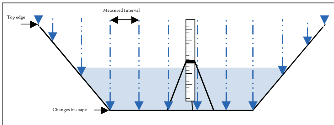
Figure 20. A basic survey method for determining the shape of the cross section by measuring the depth at marked intervals.
